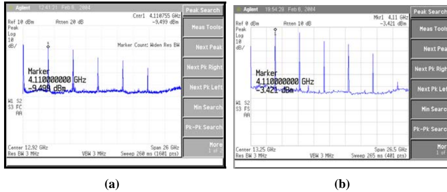
Figure 18 - RF spectrum of HML laser with 18m DSF (a), and 118m DSF (b)
